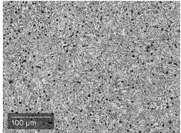
Studio System™ heat treated microstructure.
